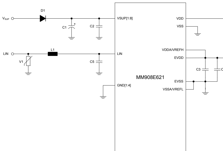
Figure 32. EMC/EMI recommendations
