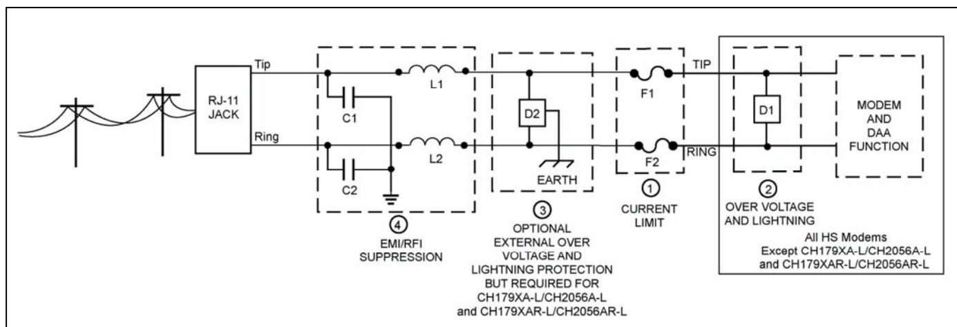
Figure 6. PSTN Line Interface for all HS Modems. CH179XA-L/CH2056A-L and CH179XAR-L/CH2056AR-L models do NOT contain internal Surge Protection (Dashed Box 2). The purchaser MUST provide external surge protection to maintain conveyed FCC Part 68 approval.
