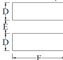
LAND PATTERNS(mm)
