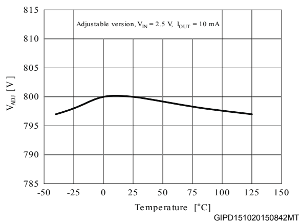
Figure 13. Output voltage vs. temperature, adjustable version
