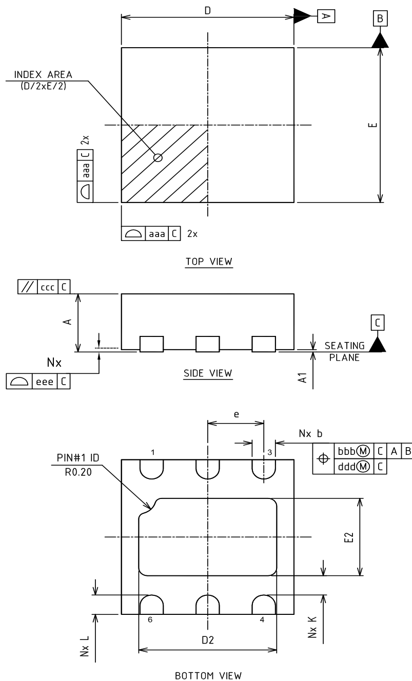
Figure 19. DFN6 (2x2) package outline
