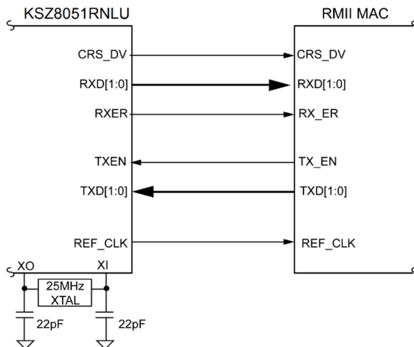
Figure 3. KSZ8051RNLU RMII Interface (25MHz Clock Mode)
