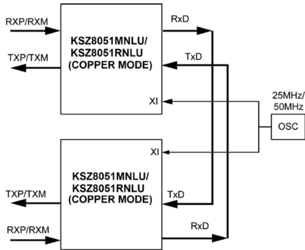
Figure 5. KSZ8051MNLU/RNLU to KSZ8051MNLU/RNLU Back-to-Back Copper Repeater
