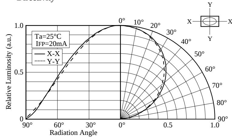
■ Directivity
