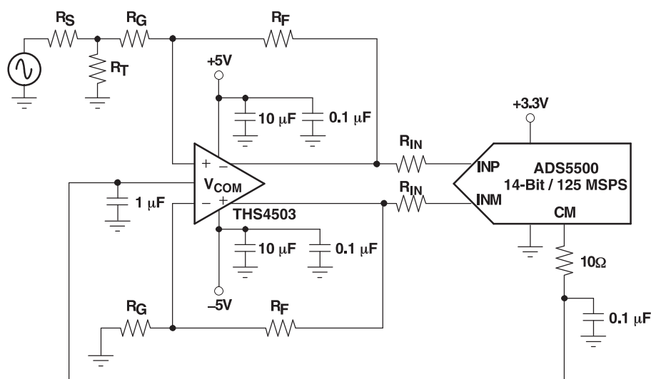
Figure 44. Using the THS4503 With the ADS5500
