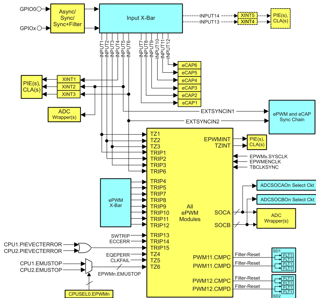
Figure 6-14. ePWM
