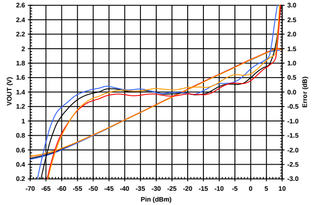
Figure 6 V_{OUT} and Log Conformance vs. Input Amplitude at 100 MHz, V_{TADJ} = 1.0\text{ V}
