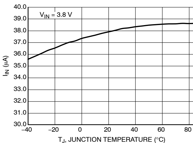
Figure 16. Supply Current vs. Temperature, 2.8 V Version
