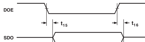
Figure 5. Serial Mode Timing for Data Output Enable and Serial Data Output ( T_{SI} = \text{Logic Low} )
