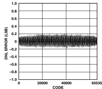
TPC 9. Differential Nonlinearity
