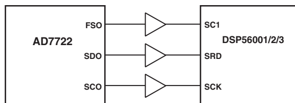
Figure 27. AD7722 to DSP56000 Interface
