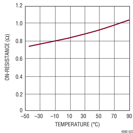
Buck Synchronous Switch (NMOS) On-Resistance vs Temperature
