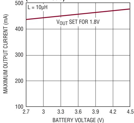
Maximum Output Current (PWM Mode)
