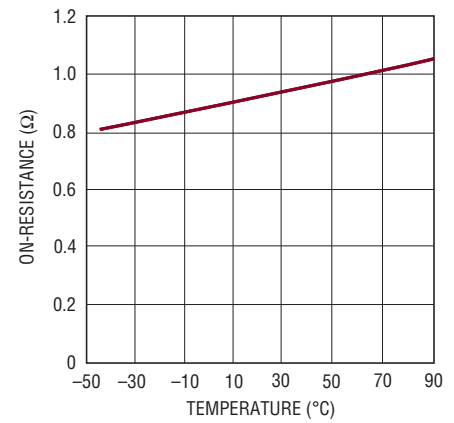
Buck Main Switch (PMOS) On-Resistance vs Temperature
