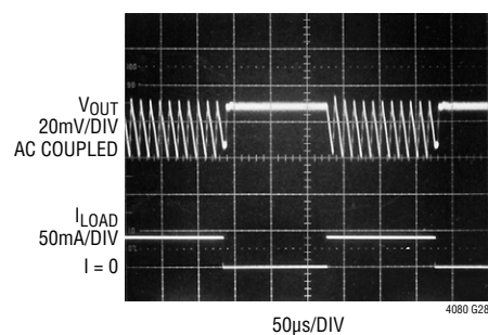
Output Voltage Transient Step Response (Burst Mode)
