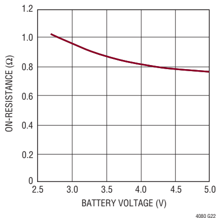
Buck Synchronous Switch (NMOS) On-Resistance vs Battery Voltage
