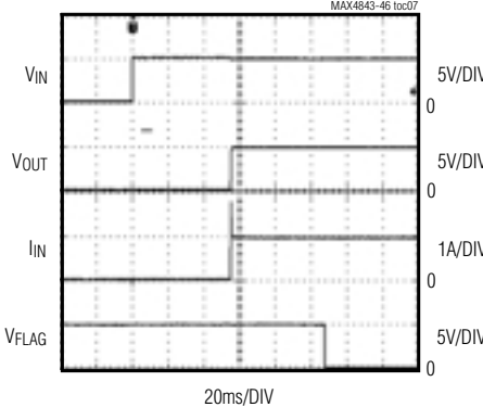
POWER-UP RESPONSE
