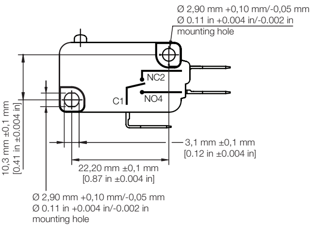
Figure 3. V15 Series USA Mounting Hole Dimensions for #4 screws
