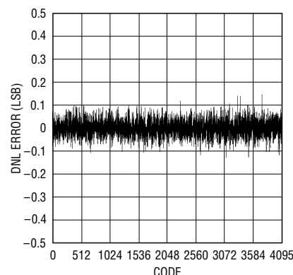
Differential Nonlinearity vs Input Code
