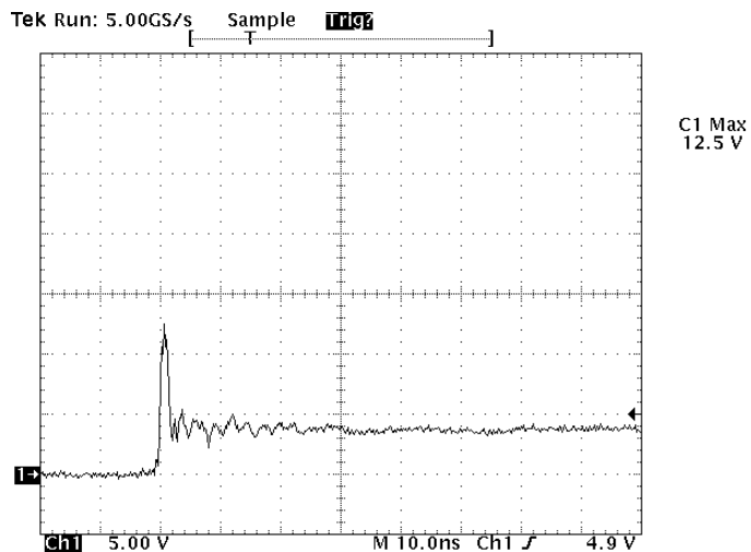
ESD Clamping (Pin 1, 2, 3, or 4 to GND) (+8kV Contact per IEC 61000-4-2)
