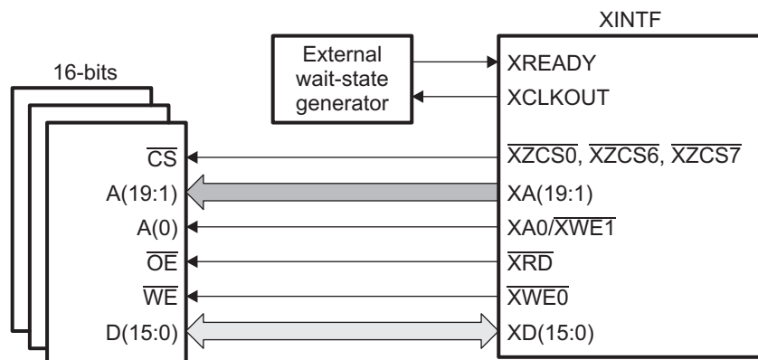
Figure 6-21. Typical 16-Bit Data Bus XINTF Connections
