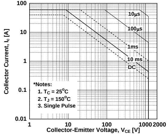
Figure 10. SOA Characteristics
