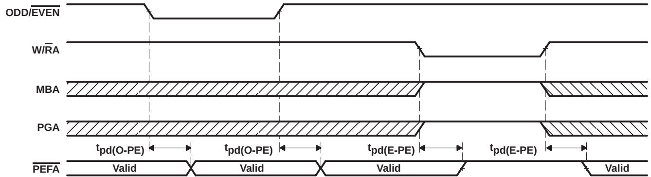
Figure 23. ODD/EVEN, W/RA, MBA, and PGA to \overline{PEFA}
