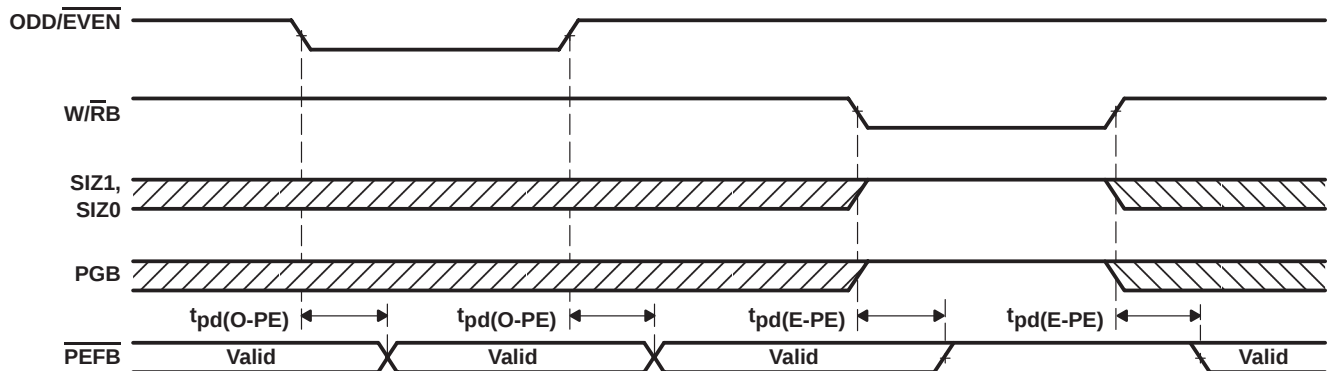
Figure 24. ODD/EVEN, W/RB, SIZ1, SIZ0, and PGB to \overline{PEFB}
