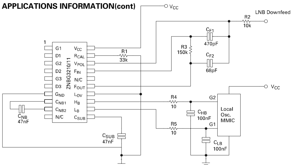
Figure 1 Lov grounded
