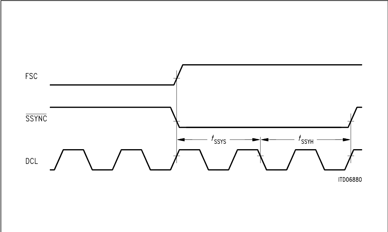
Figure 35 SSYNC Timing
