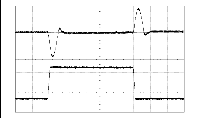
Output Load Transient Response, DLC and No NLR
