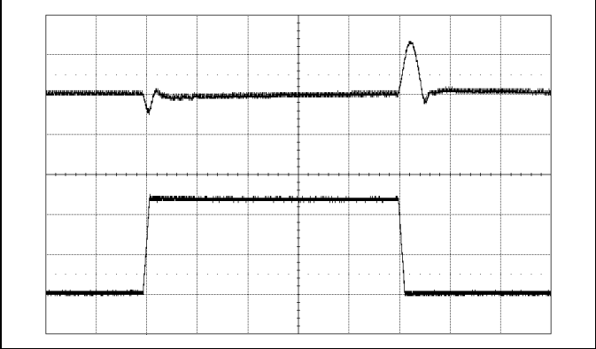
Output Load Transient Response, Default Configuration
