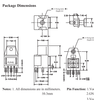
Package Dimensions
