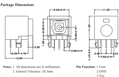
Package Dimensions
