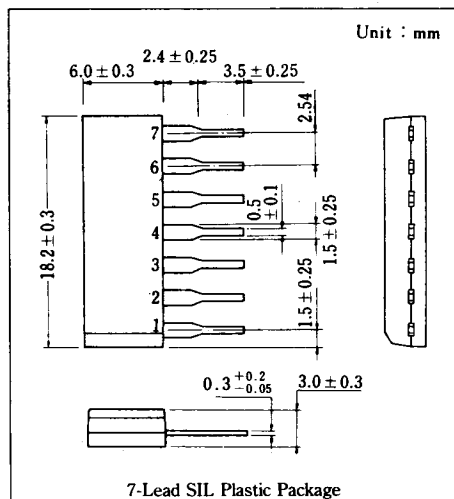
7-Lead SIL Plastic Package
