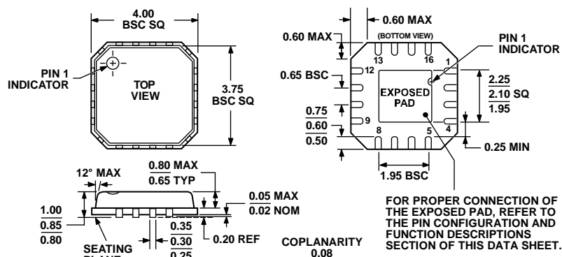
Figure 23. 16-Lead Lead Frame Chip Scale Package [LFCSP_VQ] 4 mm × 4 mm Body, Very Thin Quad (CP-16-4)
