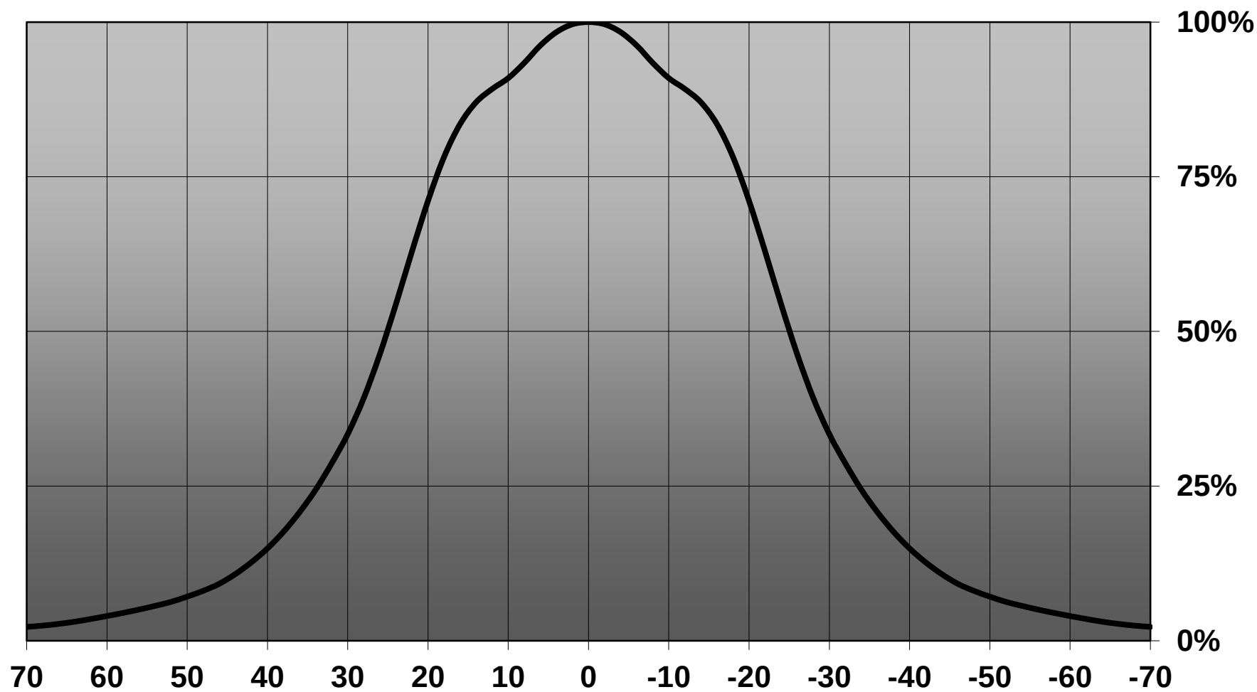
Relative intensity of C12767_HB-SQ-A (Luxeon-M)
