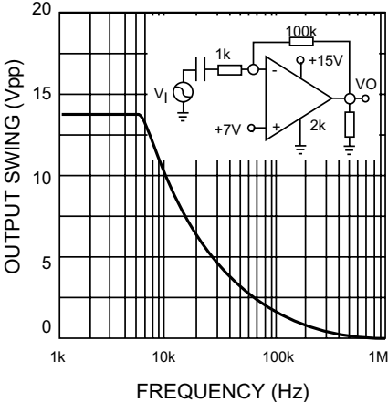
OUTPUT CHARACTERISTICS
