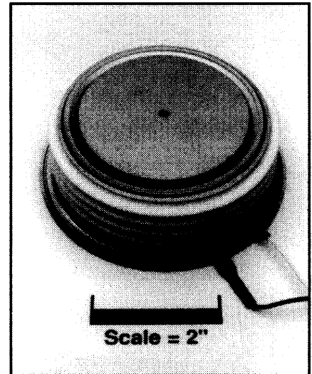
C783 Phase Control SCR 1800 Amperes Average, 3700 Volts
