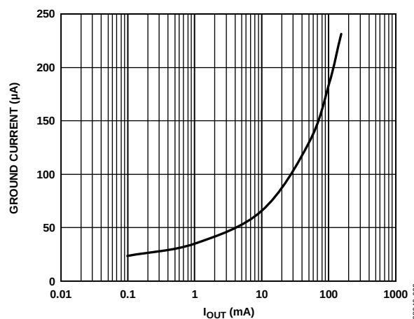
Figure 9. Ground Current vs. Load Current ( I_{OUT} )
