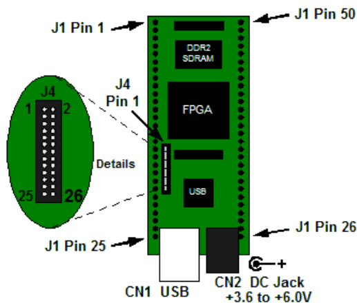
Top View (J1 Interface Headers on Bottom of PCB)
