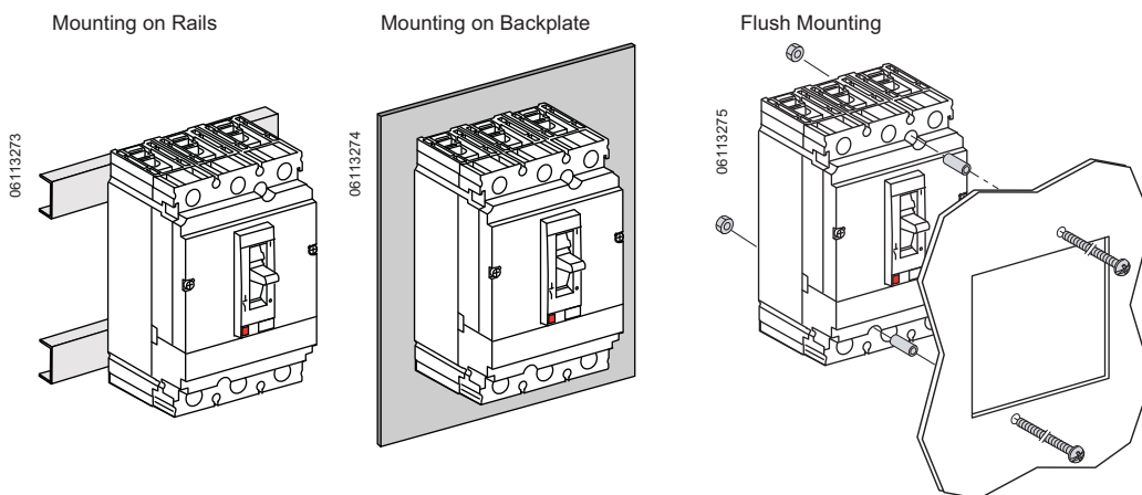
Figure 5: Unit-Mounting Options
