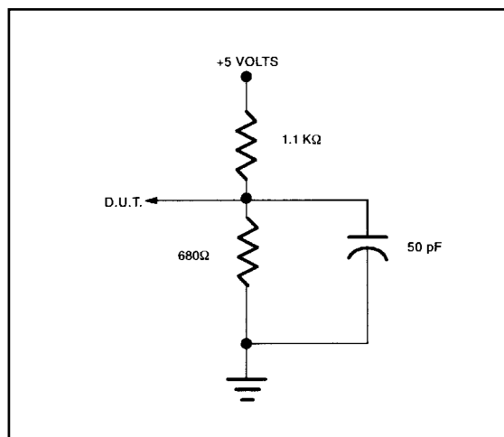
Figure 5. Output Load
