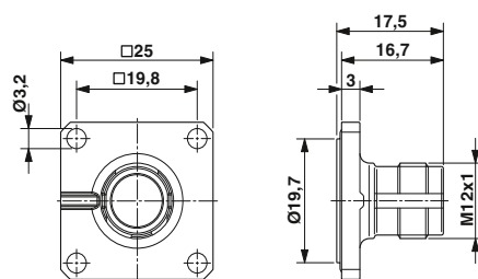
M12 square flange housing
