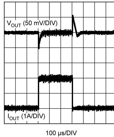
Figure 57. Transient Response
