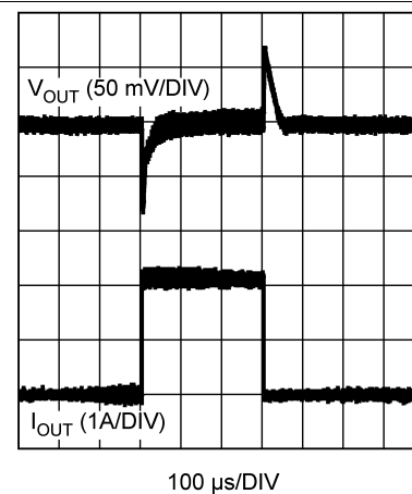
Figure 54. Transient Response
