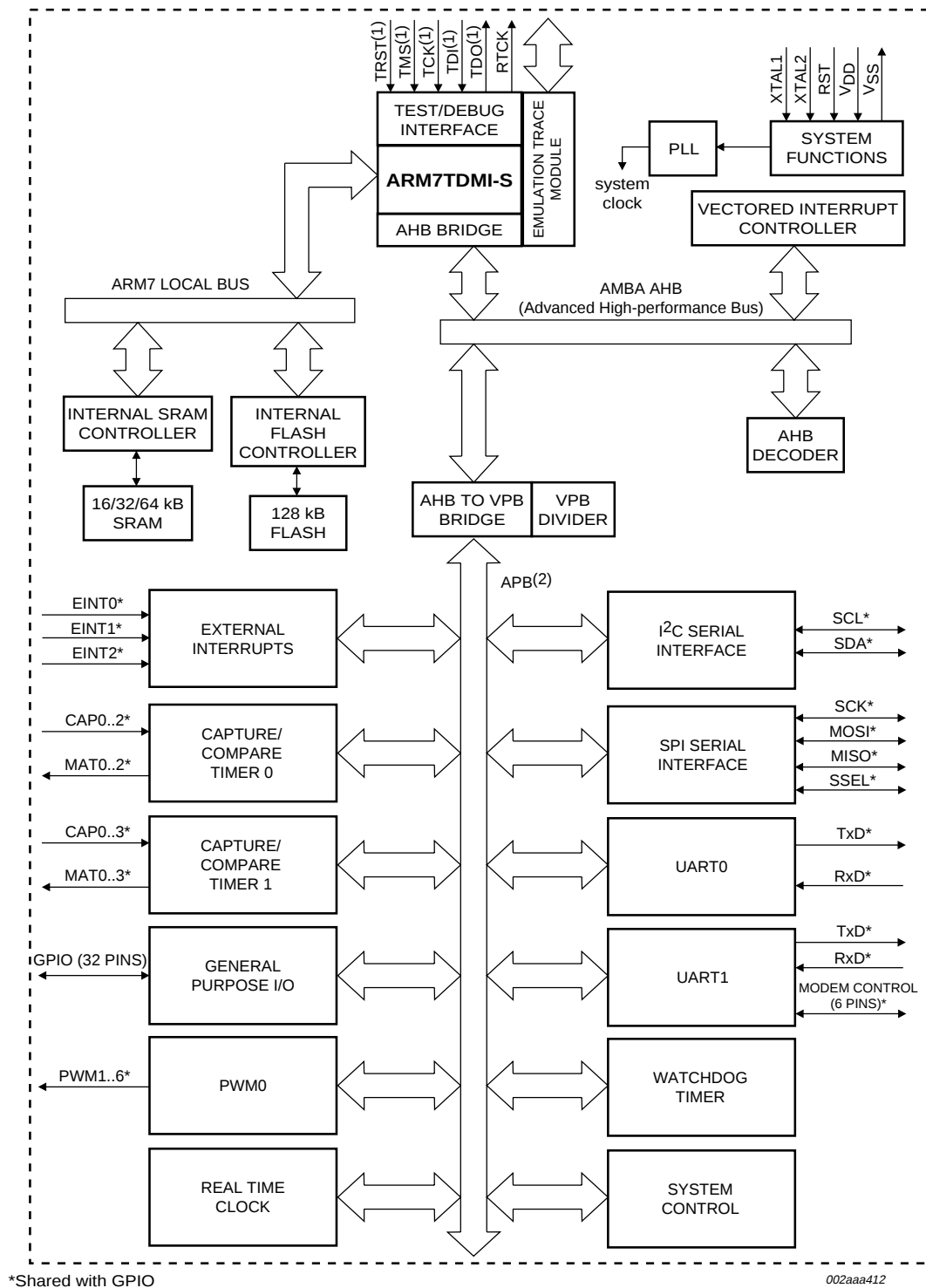
Fig 1. Block diagram.
