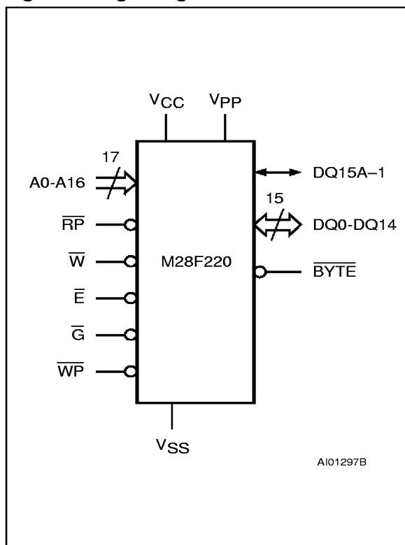
Figure 1. Logic Diagram
