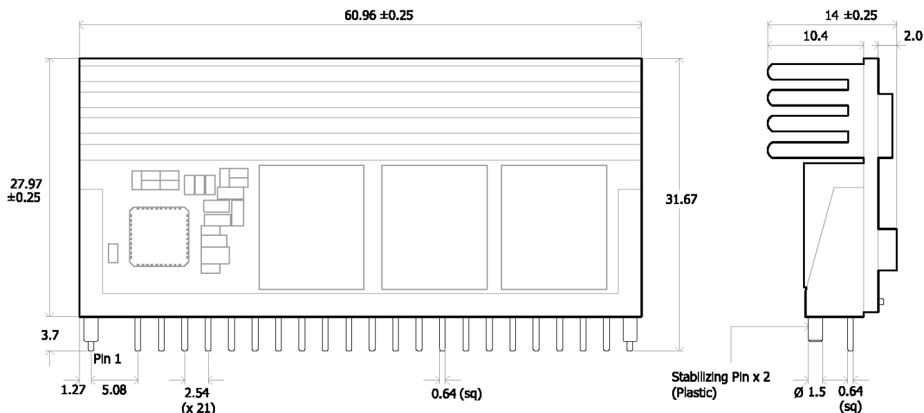
Figure 14. Mechanical Drawing
