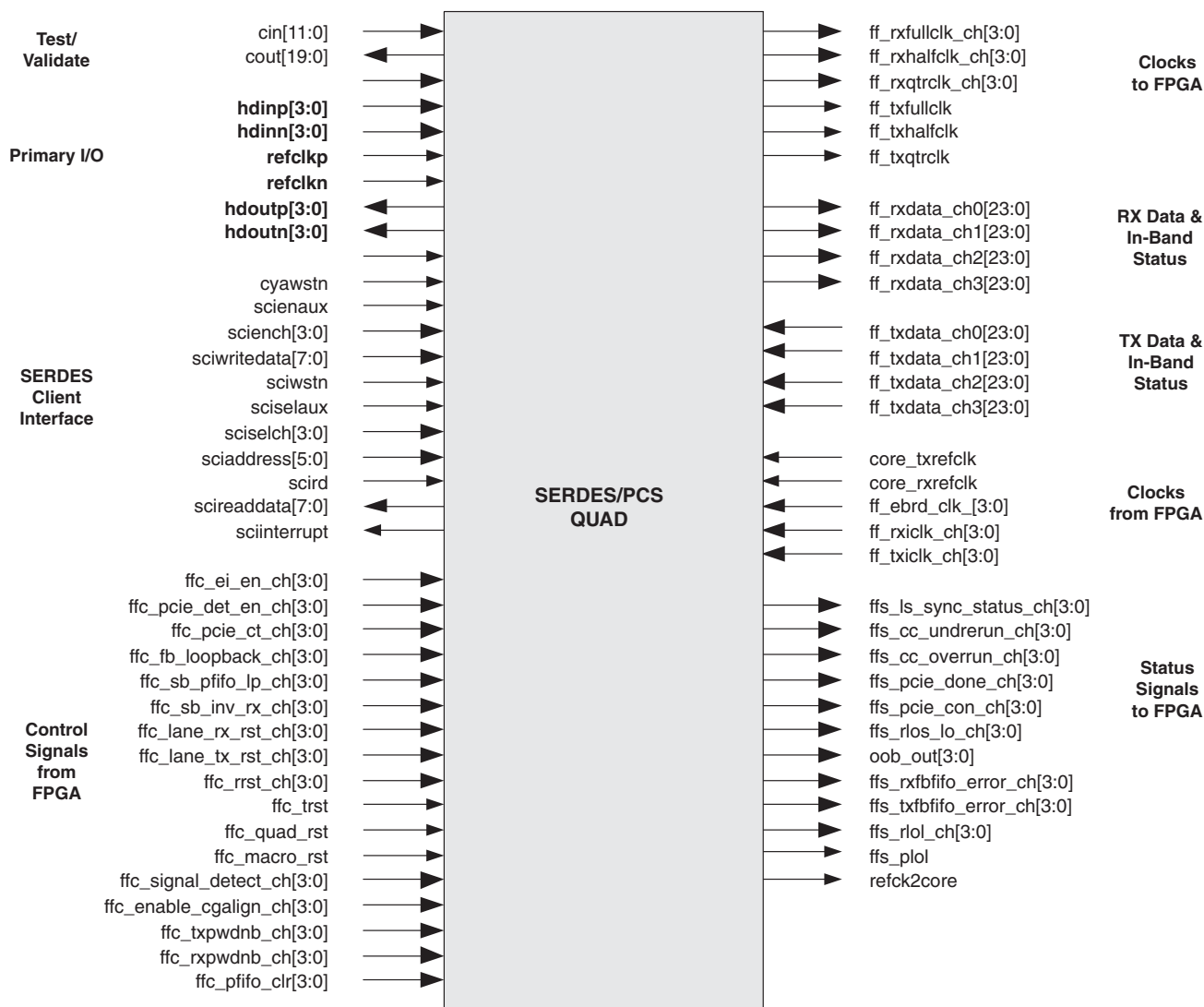
Figure 8-4. SERDES_PCS Block Signal Interface
