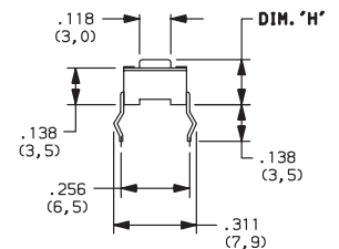
PTS635SL43 SPST
