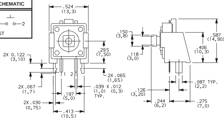
PTS125VJM73 SPST
