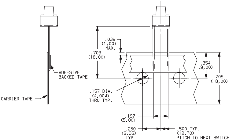
TAPE & REEL PACKAGING
