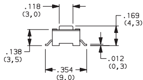
PTS635SL43SM SPST
