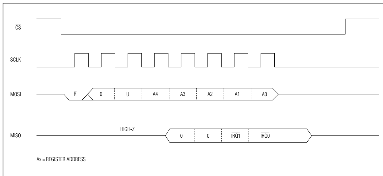
Figure 20. SPI Fast Read Cycle
