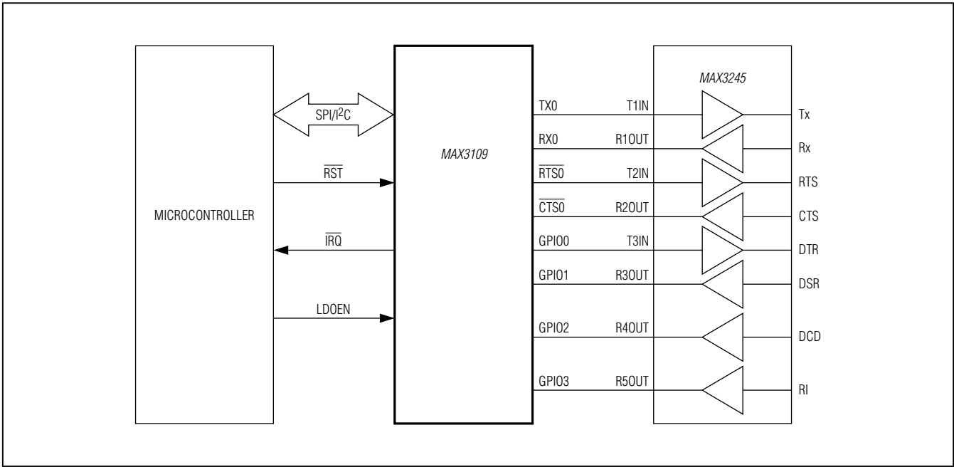
Figure 30. RS-232 Application
