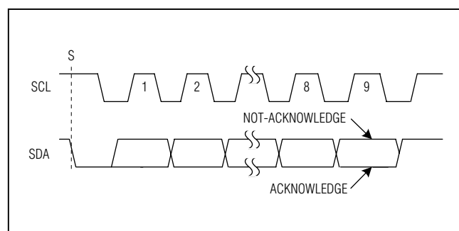
Figure 26. Acknowledge
