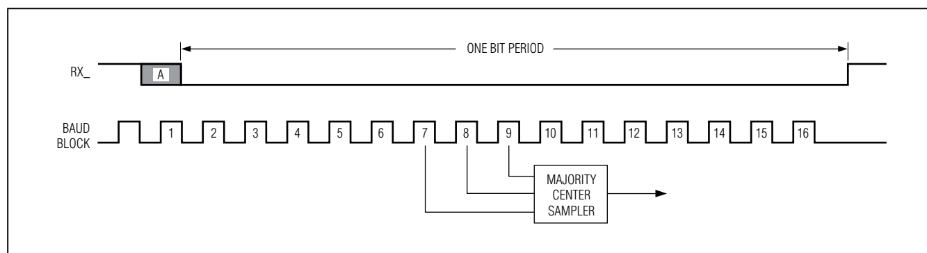
Figure 6. Midbit Sampling
