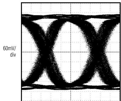
EQUALIZER OUTPUT EYE AFTER 30in OF FR-4 (K28.5 AT 12.5Gbps)
