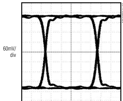
EQUALIZER OUTPUT EYE AFTER 30in OF FR-4 ( 2^7 PRBS WITH 100 CIDs AT 3.2Gbps)
