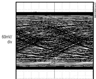
EQUALIZER INPUT EYE AFTER 30in OF FR-4 ( 2^7 PRBS WITH 100 CIDs AT 10.7Gbps)
