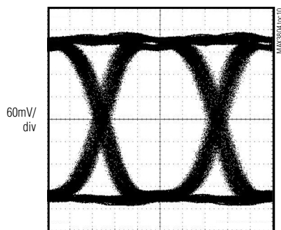
EQUALIZER OUTPUT EYE AFTER 24ft OF RG-188/U COAXIAL CABLE, SINGLE ENDED ( 2^7 PRBS WITH 100 CIDs, 9.953Gbps)
