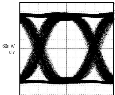
EQUALIZER OUTPUT EYE AFTER 30in OF FR-4 ( 2^7 PRBS WITH 100 CIDs AT 10.7Gbps)
