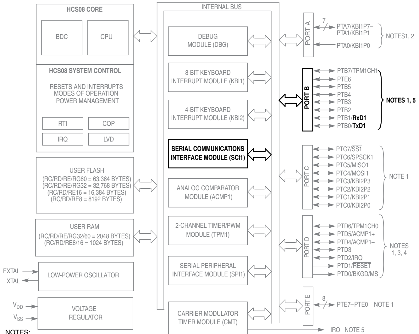
Figure 11-1. MC9S08RC/RD/RE/RG Block Diagram Highlighting SCI Block and Pins
