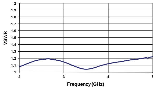
VSWR ( 2-5 GHz )
