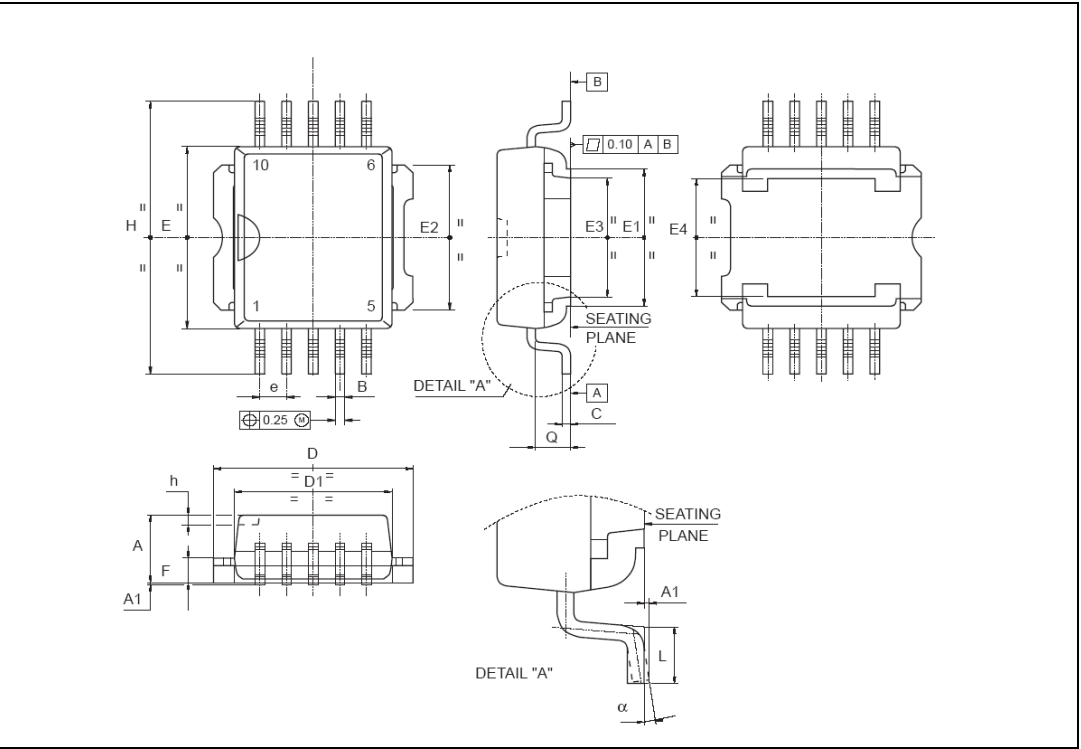
Figure 26. Package dimensions
