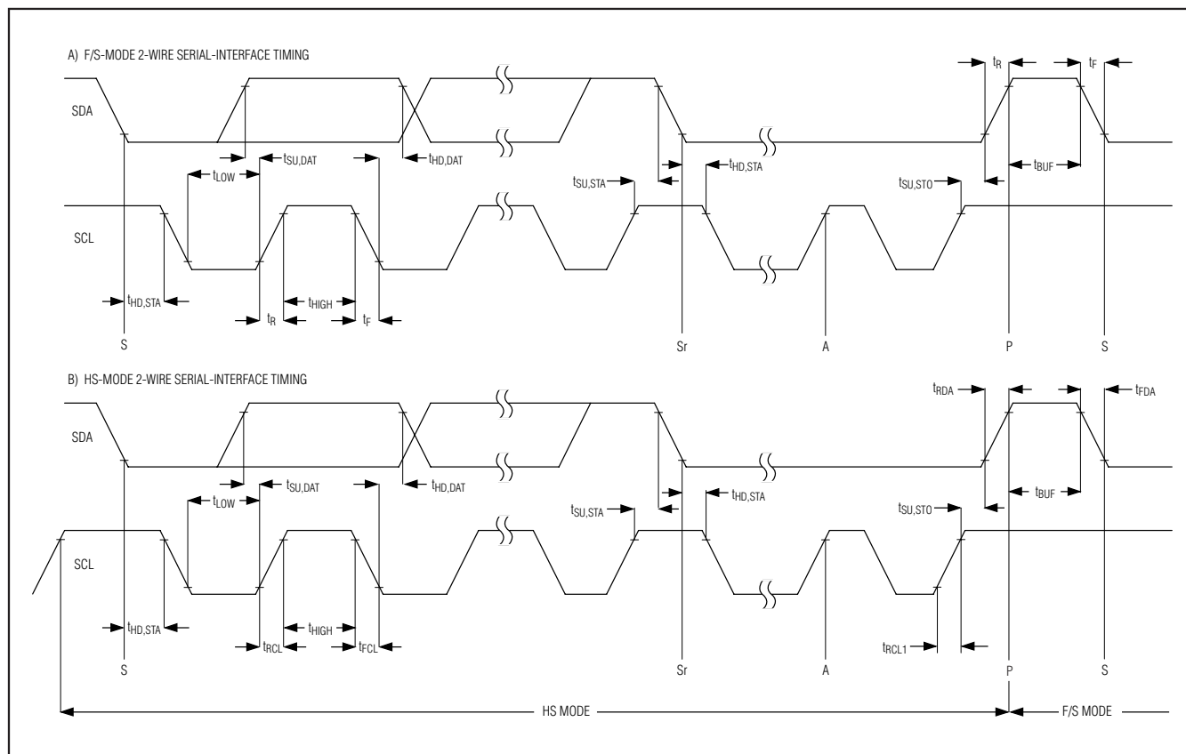
Figure 1. 2-Wire Serial-Interface Timing
