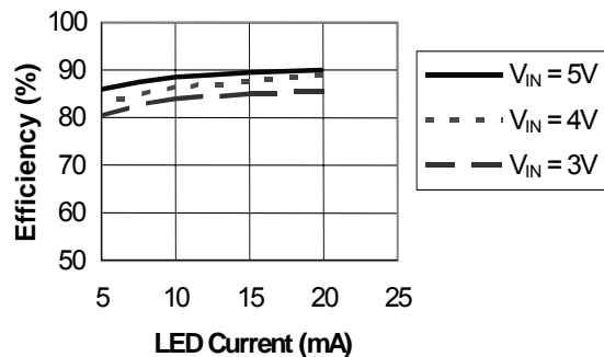
Efficiency vs LED current, 1 string of 6 Using Toko D62CB 47μH Inductor
