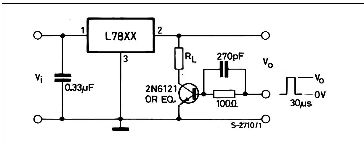
Figure 2 : Load Regulation
