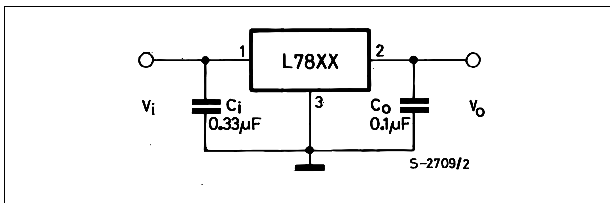
Figure 2 : Load Regulation
