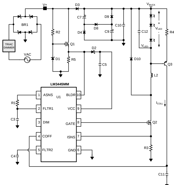
Typical LM3445 LED Driver Application Circuit
