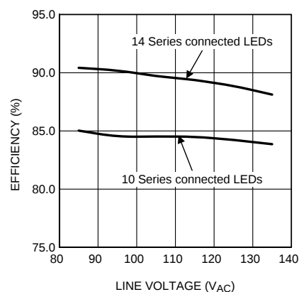
Efficiency vs Line Voltage
