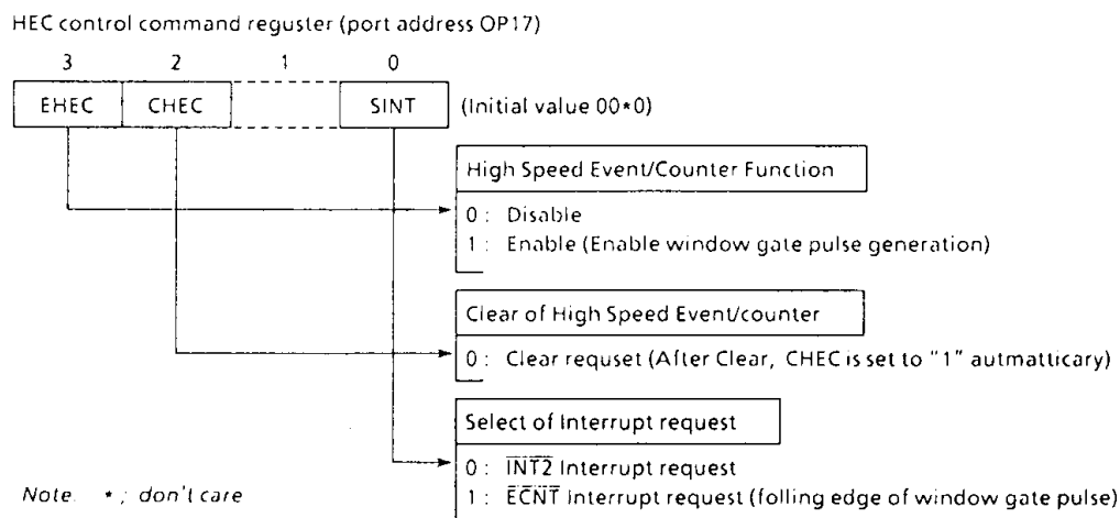
Figure 2-13. HEC Control Command Register
