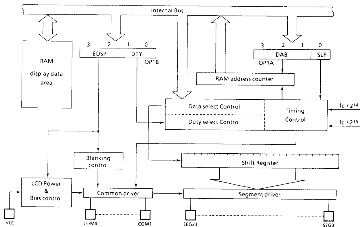
Figure 2-3. Configuration of LCD driver
