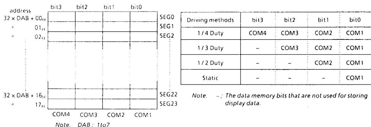
Figure 2-6. The correspondnce between the display data area and the SEG/COM pins.
