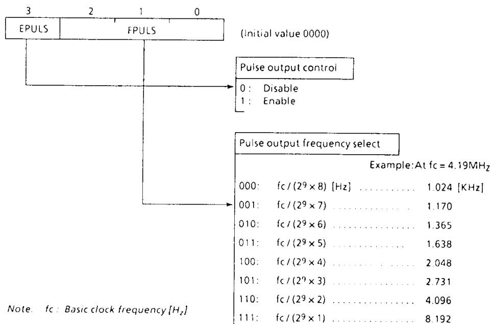
Figure 2-17. Pulse output command register
