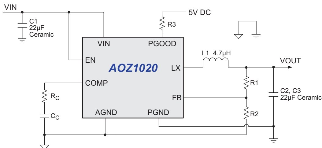
Figure 1. 3.3V/2A Buck Regulator
